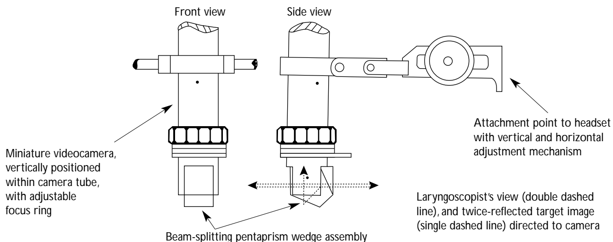
Figure 3. Optical path of the Airway Cam direct laryngoscopy video system. Figure courtesy of Airway Cam Technologies, Inc., Wayne, PA.
